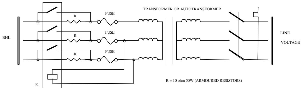
Fig 1: Wiring for a line transformer or autotransformer with rated power > 6kVA
