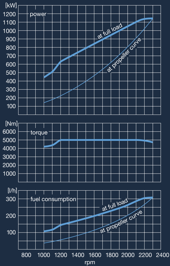
■ V12 -1550 CRM, 1,140 kW (1,550 mhp)
