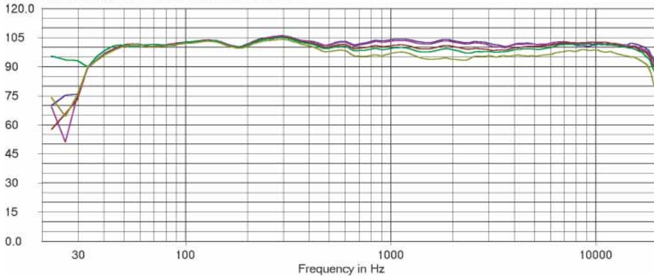
H3 Horizontal Magnitude in dB SPL/2.83V at 1 meter
