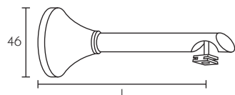
2532-- Supporto Träger Bracket Soporte Support Wspornik
