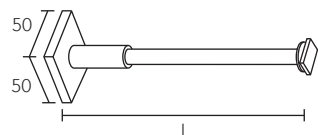
3133-- Supporto Träger Bracket Soporite Support Wspornik
