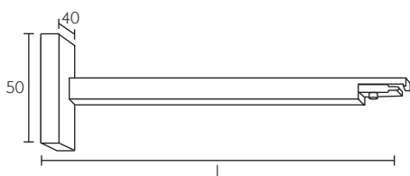
2233-- Supporto Bracket Support
